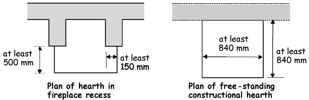
Figure 3.43 Hearth construction
