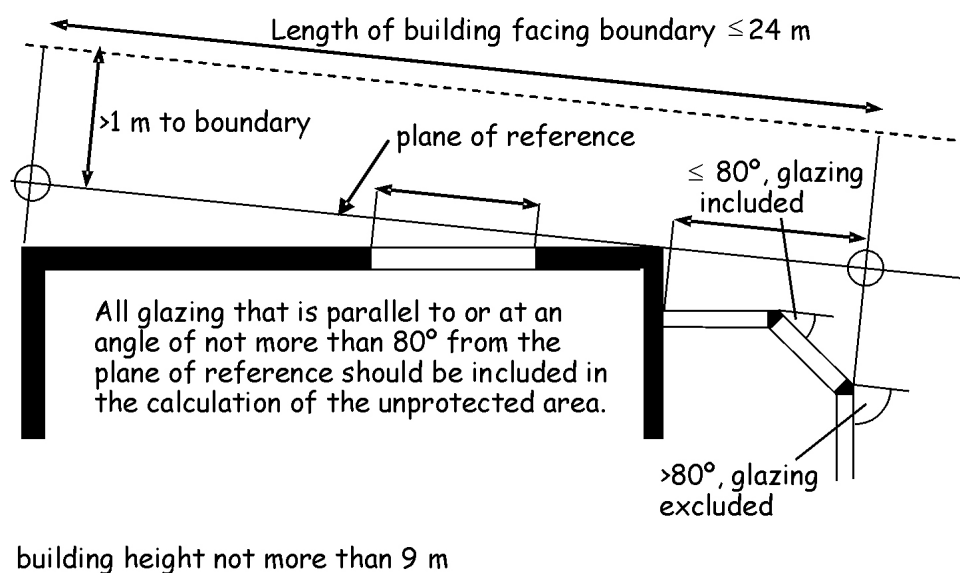
Figure 2.3 Conservatory example
