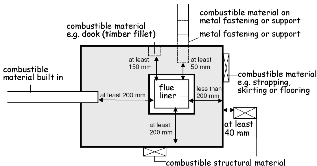
Figure 3.38 Plan view of masonry chimney
