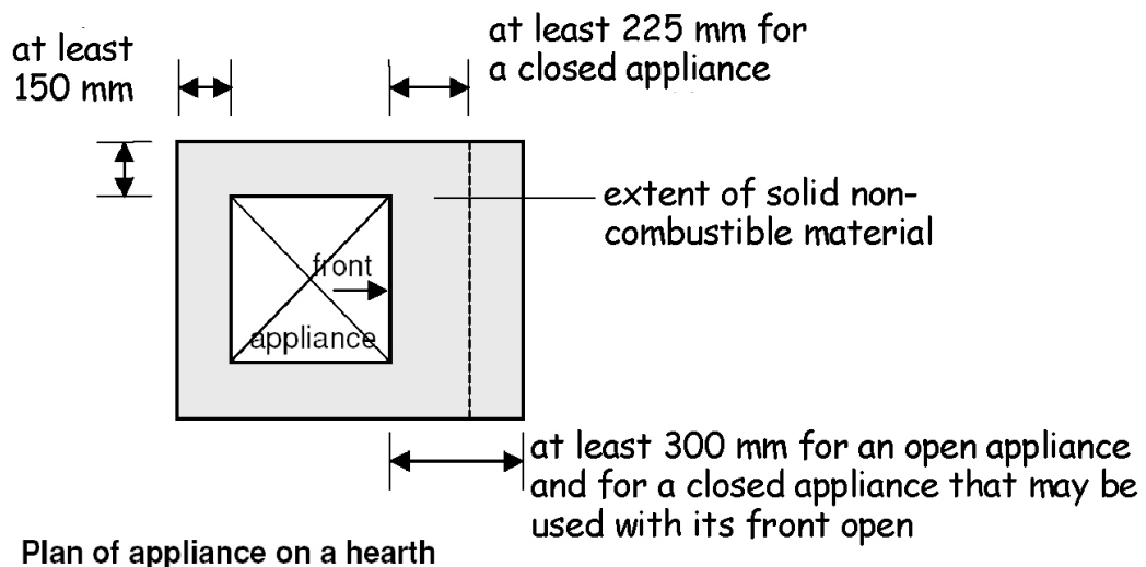
Figure 3.44 Appliance location
