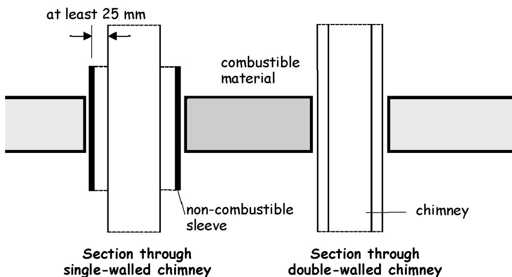
Figure 3.40 Section through single-walled Chimney (vertical)
