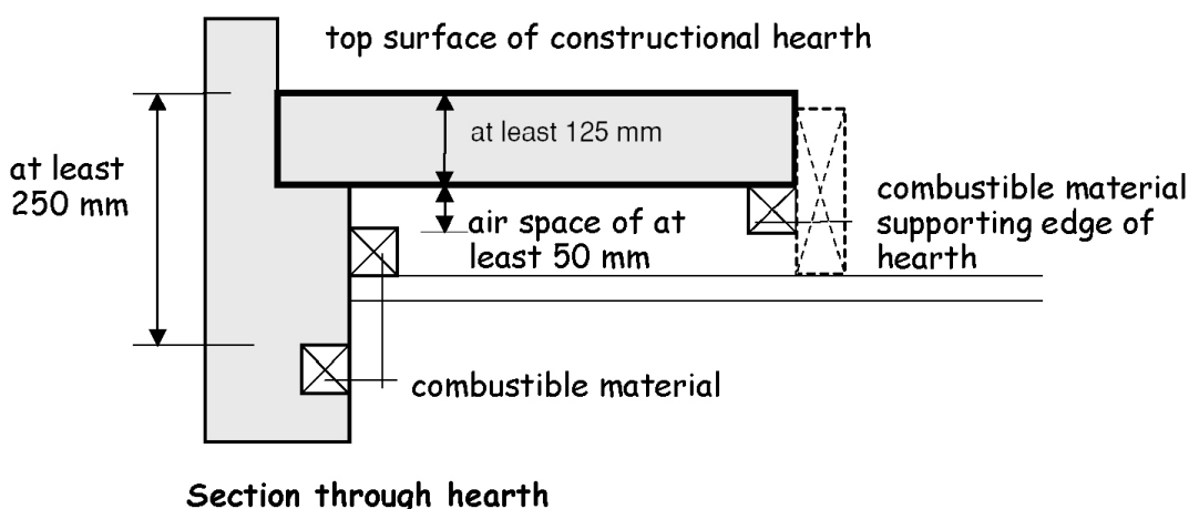
Figure 3.50 Section through hearth
