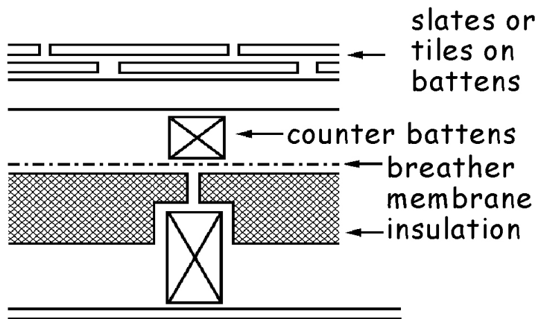
Figure 3.27 Roof constructions - Type C (slate or tiles - insulation on decking)
